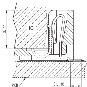
For pins 20, 28, 44, 52, 68, 84
