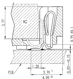
IC160Z-0**4-24** (Type 1)
