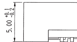
Height Dimension Rectangle Form (both terminal types)
